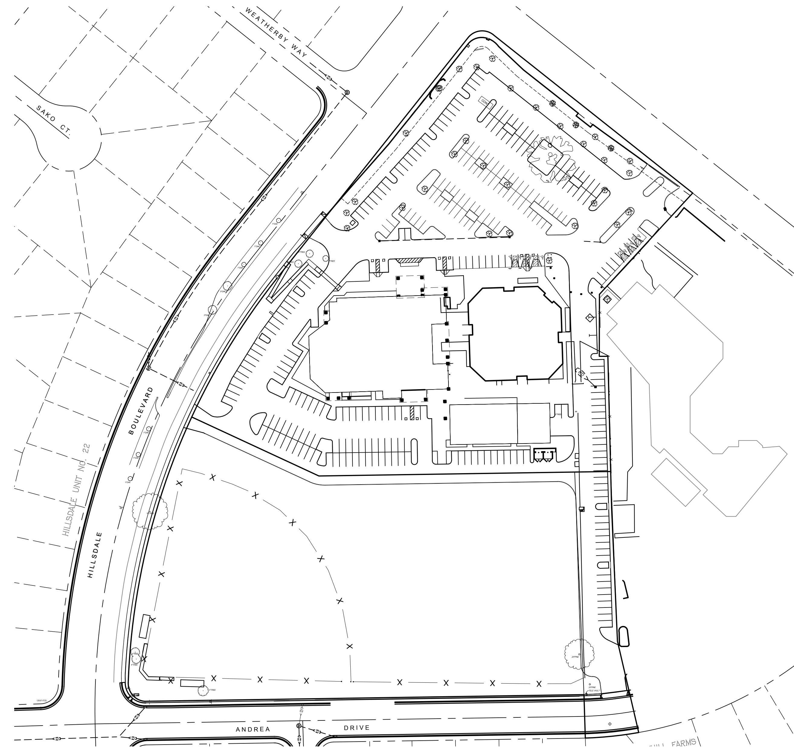
PROJECT SITE PLAN SCALE: 1"=80'
